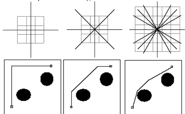
Figure 7: 3 distance metrics and resulting paths. L1 allows 4 distinct directions of movement. L2 allows 8, L3 allows 16. We used L4 which allows 32 directions.
