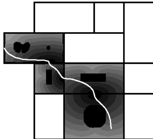
Figure 8: An eventual path from left middle, to middle bottom through 5 rooms of the museum. The navigation function that was used for each room is pictured. Usually the navigation is chosen for a room is the one generated that leads to the exit door of that room. In the final room, the algorithm is run backwards and calculates a path from the destination location to the entry room. The resultant path is reversed and combined with the other paths.
